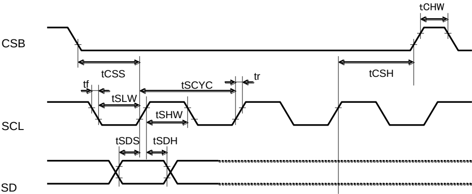
Figure 4. Interface Timing
