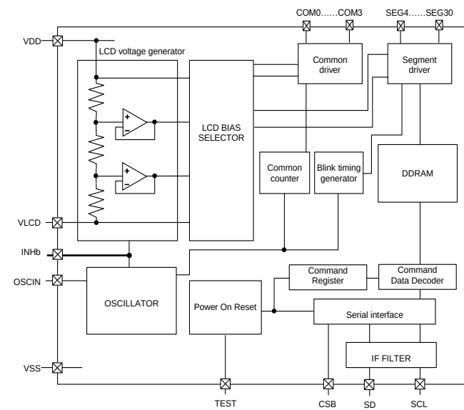
Figure 2. Block Diagram
