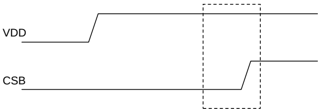
Figure 22. CSB Timing
