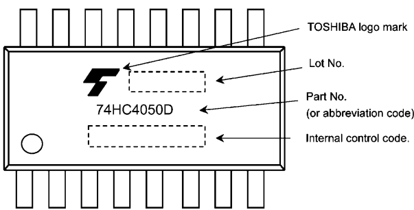
74HC4050D
