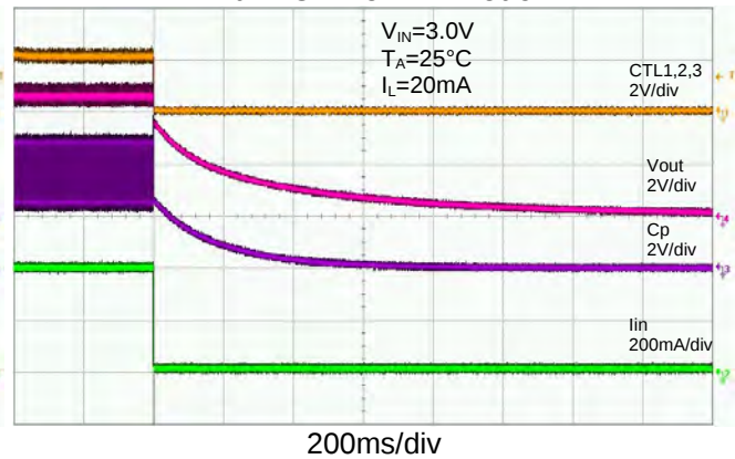
Turn-Off from 2x Mode
