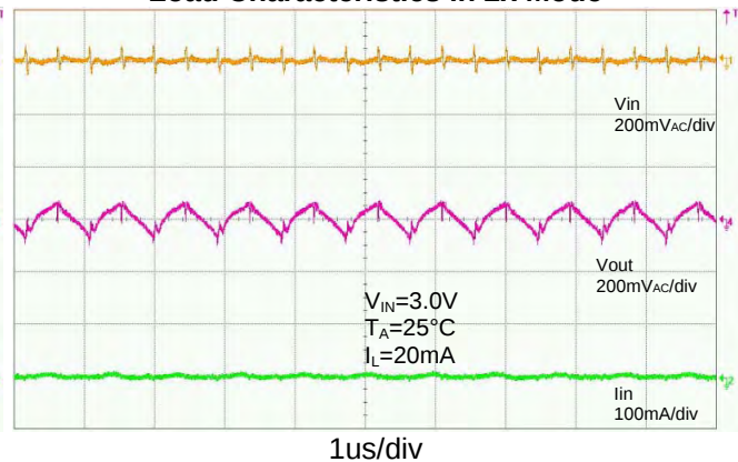
Load Characteristics in 2x Mode
