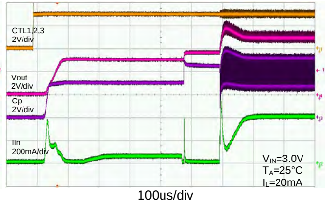
Turn-On to 2x Mode
