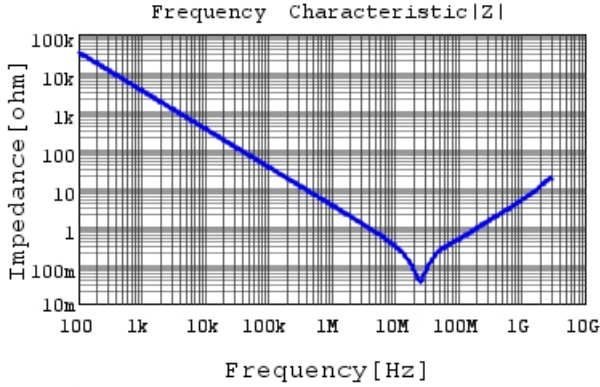
GRM31CR72E473KW03 |Z| DCOV, 25degC
