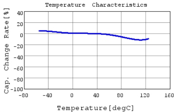
GRM31CR72E473KW03 C-Temp. capchange, DCOV, 1
