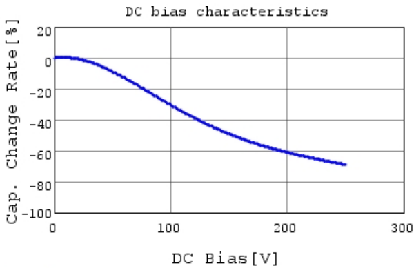
GRM31CR72E473KW03 C-DC bias capchange, 25.0c
