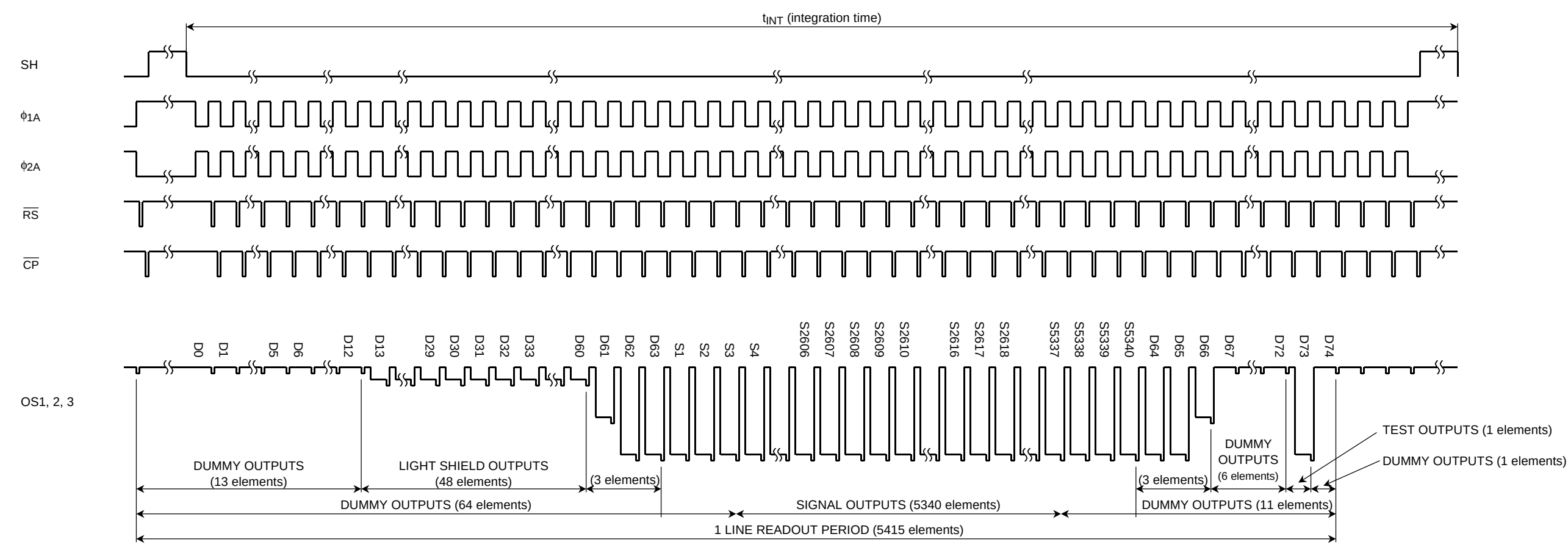
Timing Chart 1: Bit Clamp Mode
