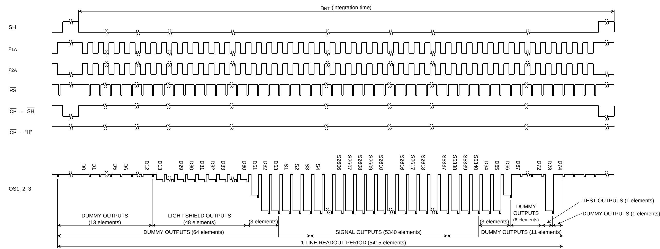
Timing Chart 2: Line Clamp Mode
