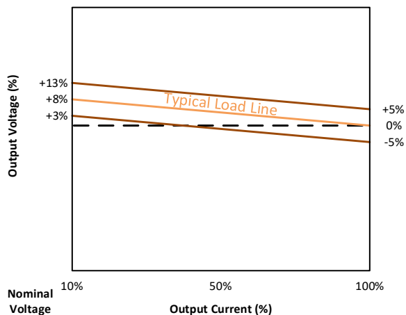
Tolerance Envelope Graph
