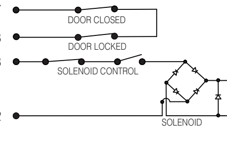
Figure 9. Wiring Schematic Series Connection (4-pin Terminal)
