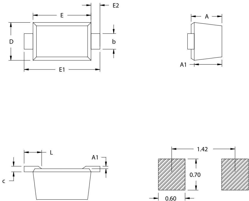
Recommended Footprint
