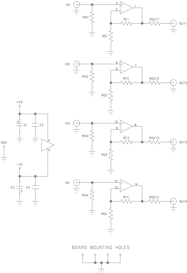
Figure 10. CEB018 Schematic
