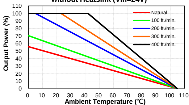
CQB200-24S Derating Curve without Heatsink (Vin=24V)
