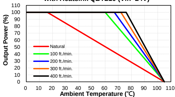
CQB200-24S Derating Curve with Heatsink QBT210 (Vin=24V)
