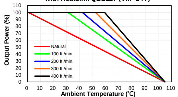
CQB200-24S Derating Curve with Heatsink QBL127 (Vin=24V)
