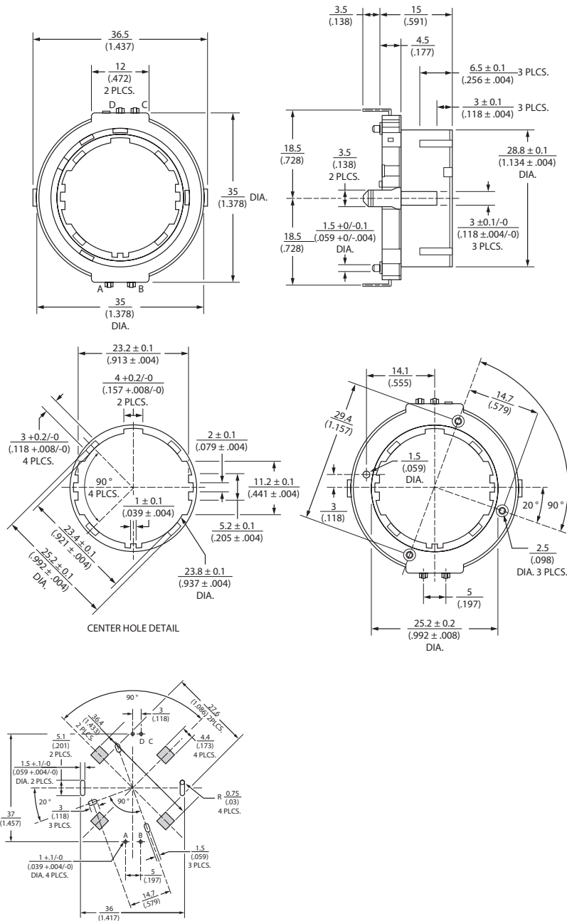
Recommended PCB Layout Top View
