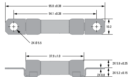
ZXBBD Bolt Down (Axial)
