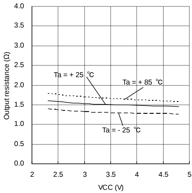
Figure 4. Output resistance
