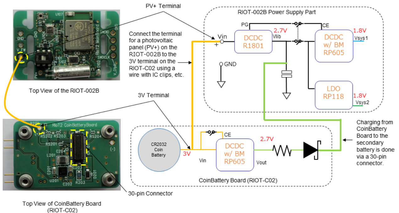
Figure 3. Connection between 3V Terminal of Coin Battery Board and PV+ Terminal of RIOT-002B
