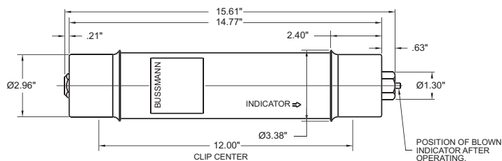
MV055F1DAX
