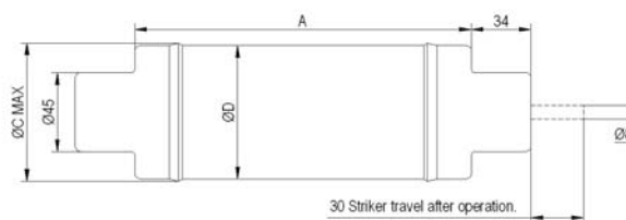
Dimensions - mm
