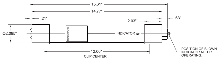
MV055F1CAX
