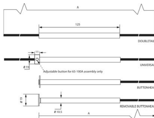
60-100A
