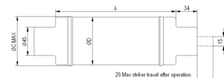
SJ Fuses
