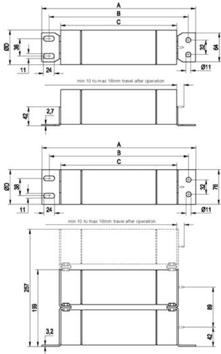
Tag type '0'
