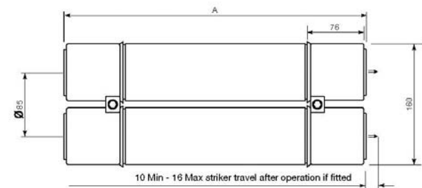
K Tags (double barrel fuse links)
