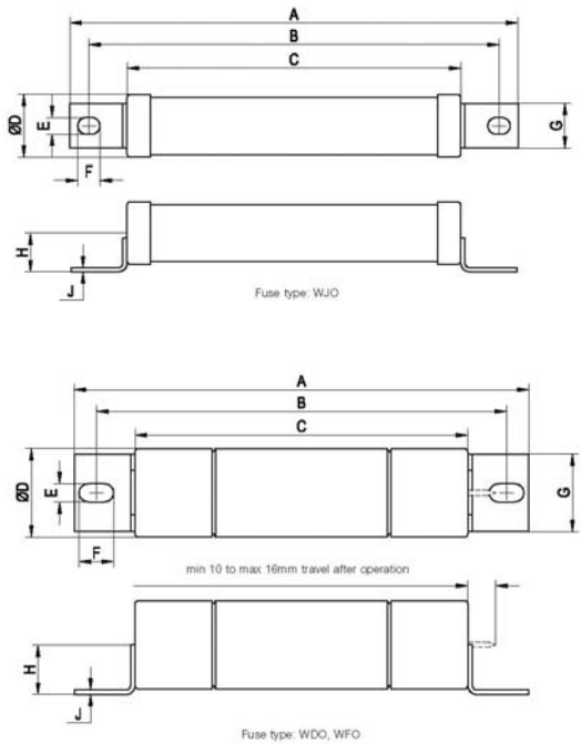
Tag type '6'
