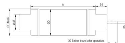
EJ Fuses
