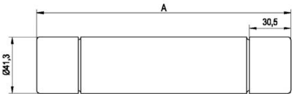
Dimensions - mm
