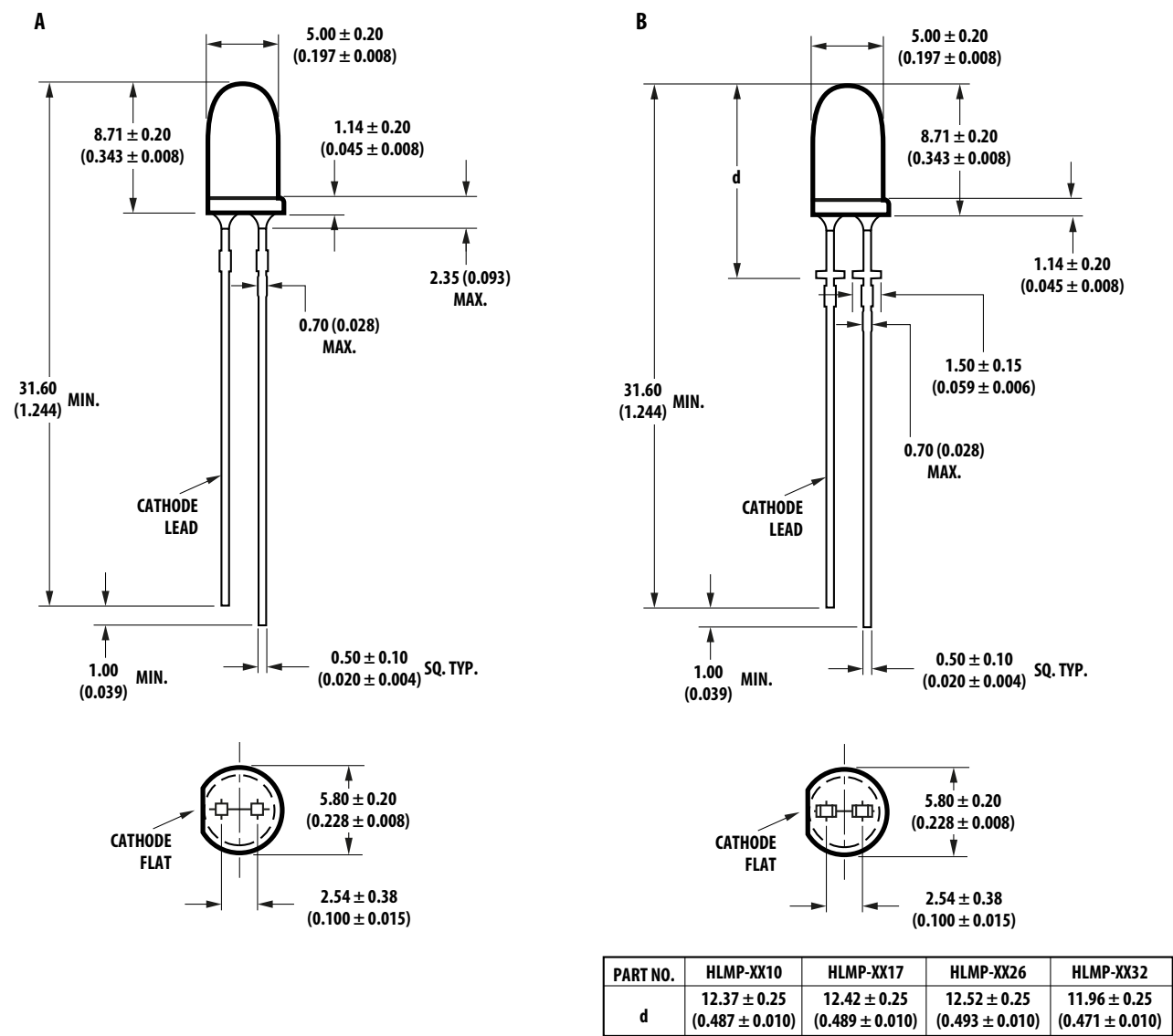
Figure 1: Package Dimensions
