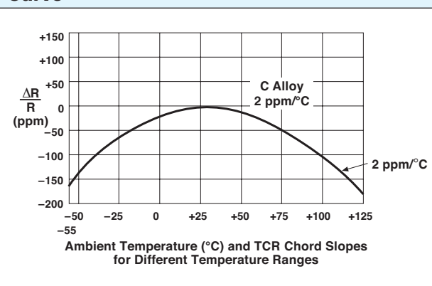
Figure 4 – Typical Resistance/Temperature Curve
