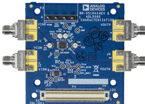
Figure 1. ADL5580-EVALZ , Top
