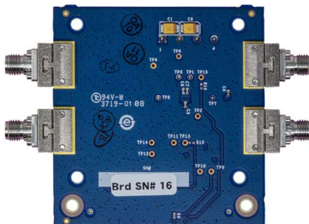
Figure 2. ADL5580-EVALZ , Bottom
