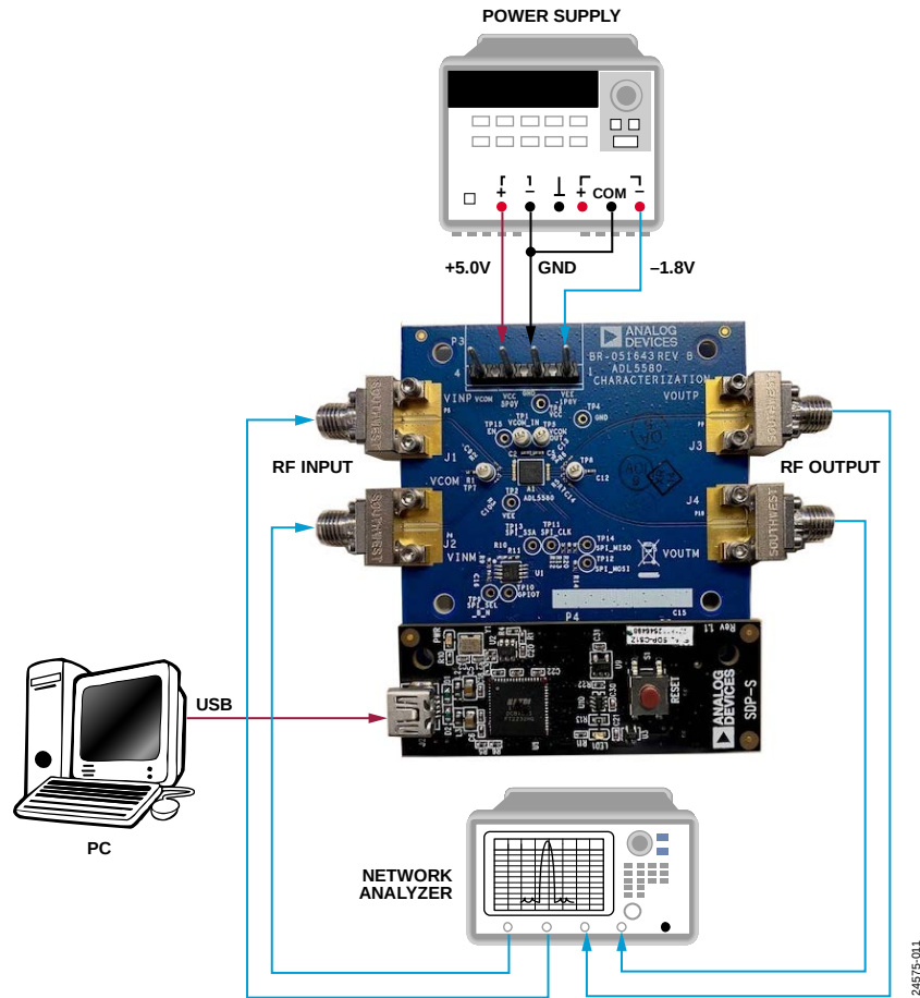
Figure 4. ADL5580-EVALZ Connection Diagram
