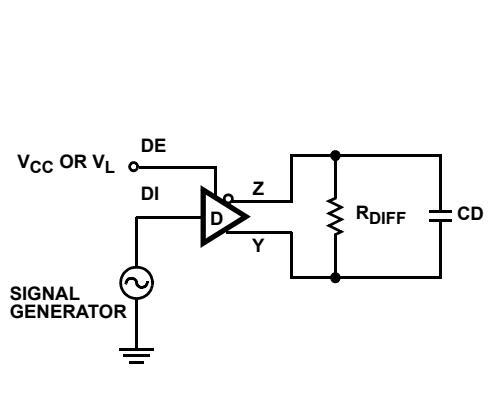
FIGURE 5A. TEST CIRCUIT
