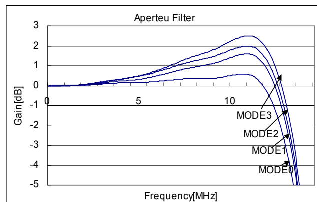
Fig. 42 Aperture Filter
