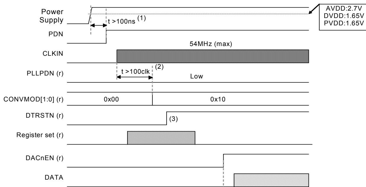
Fig. 15 Power-Up sequence (To set High Speed Video DAC mode after power-up)
