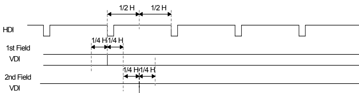
Fig. 157 HD/VD timing
