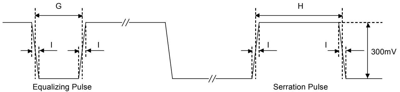
Fig. 126 Equalizing Pulse と Serration Pulse
