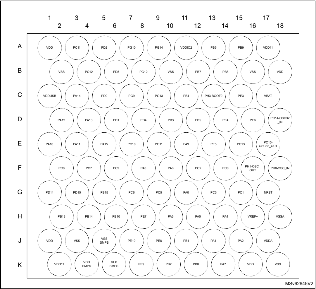
Figure 13. WLCSP90-SMPS ballout
