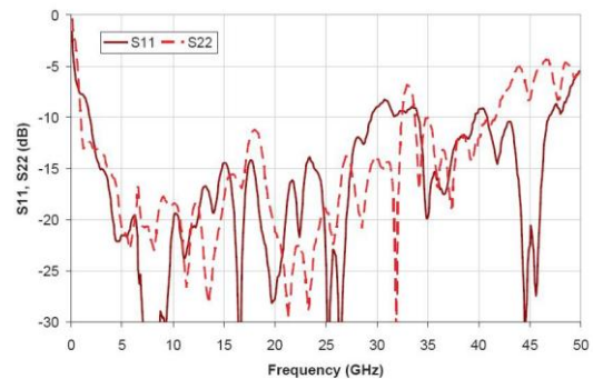
UA2V50LM S11, S22
