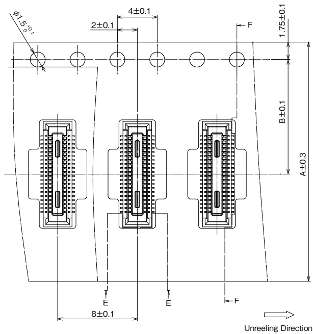
Embossed Tape Dimensions
