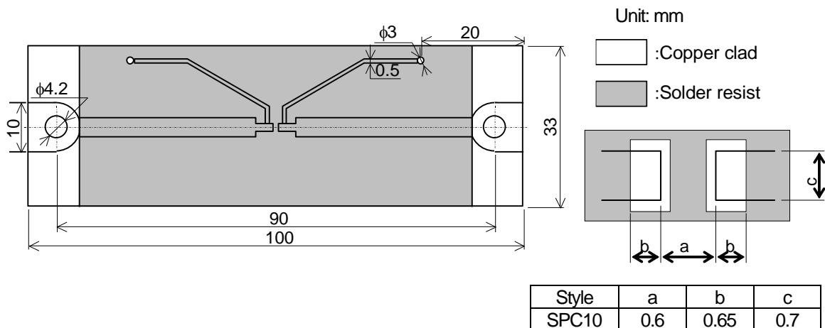
Figure-2 SPC TEST SUBSTRATE
