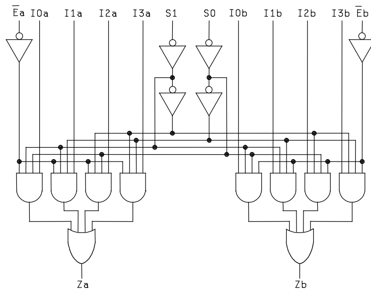
FIGURE 2. Logic diagrams.
