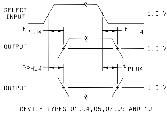
FIGURE 4. Switching time waveform - Continued.
