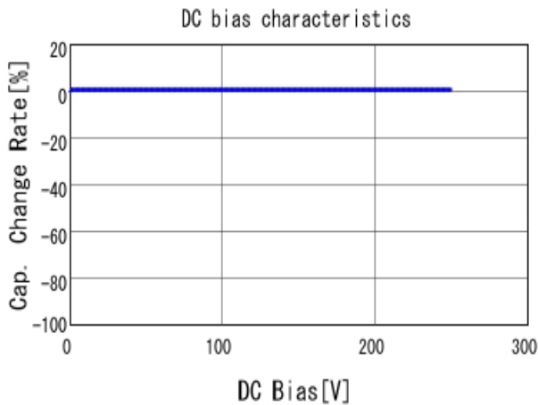
■ DE1B3KX471KN4AN01F C-DC bias capchange, 20.0degC, AC1
