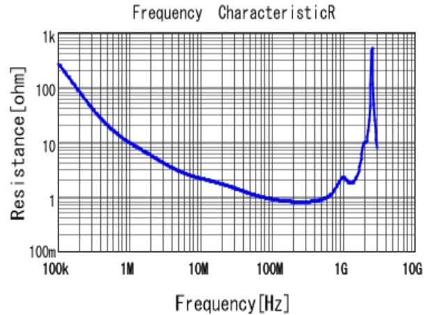
■ DE1B3KX471KN4AN01F R DC0V, 20degC
