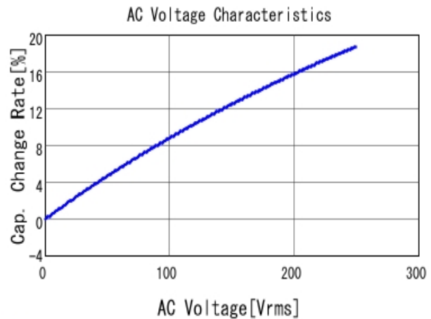
■ DE1B3KX471KN4AN01F C-AC Voltage capchange, DC0V, 20.0
