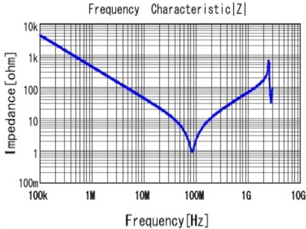
■ DE1B3KX471KN4AN01F |Z| DC0V, 20degC
