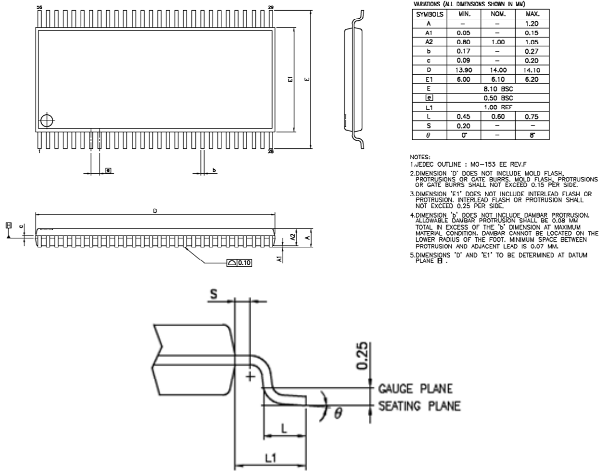
Figure 15. Package Diagram
