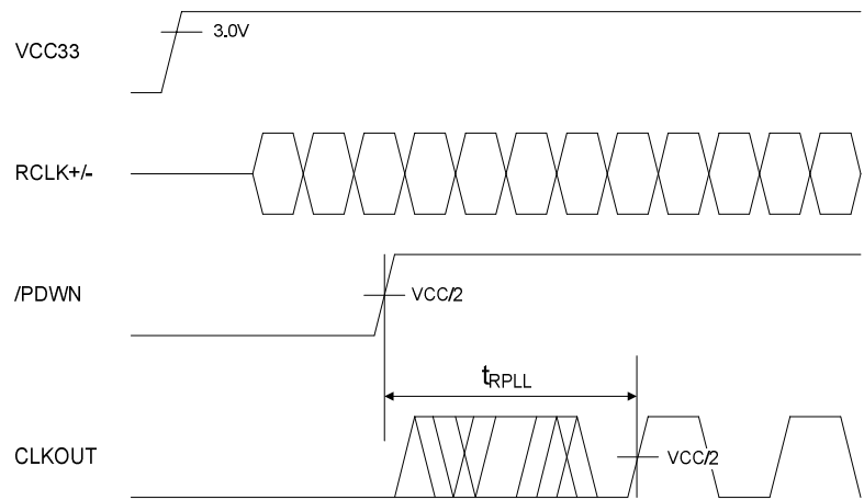
Figure 11. PLL Lock Loop Set Time
