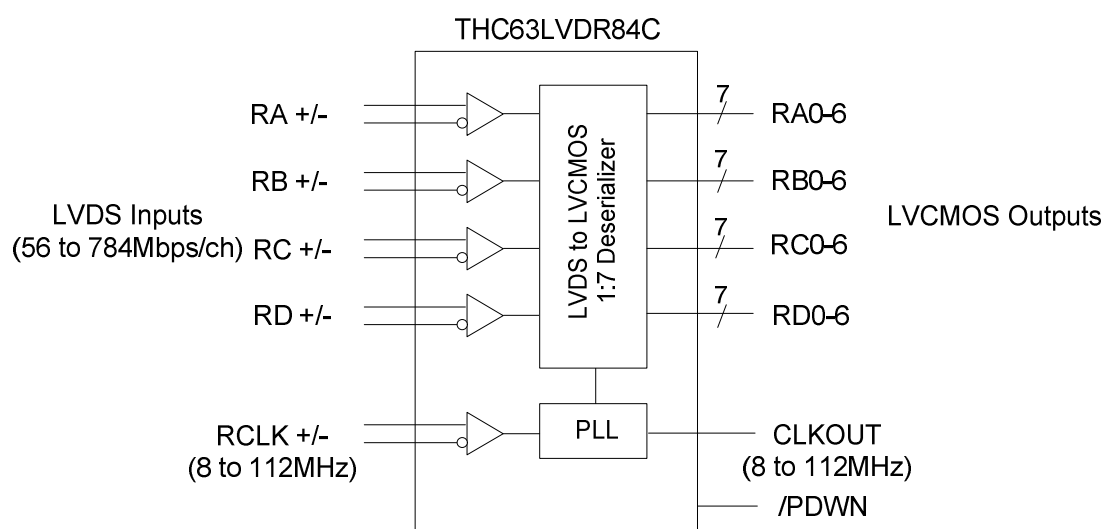
Figure 1. Block Diagram
