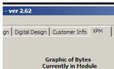
Fig 4: XPM Tab
