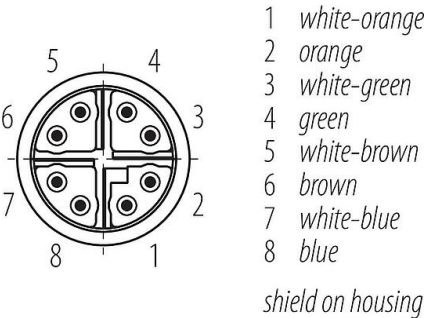
Contact arrangement (Plug-in side)
