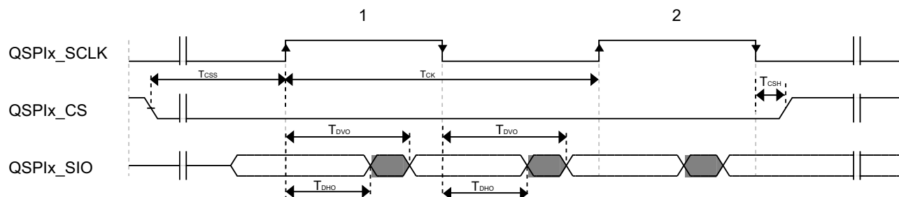
Figure 38. QuadSPI output/write timing (DDR mode)
