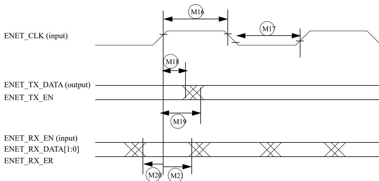
Figure 17. RMII mode signal timing diagram
