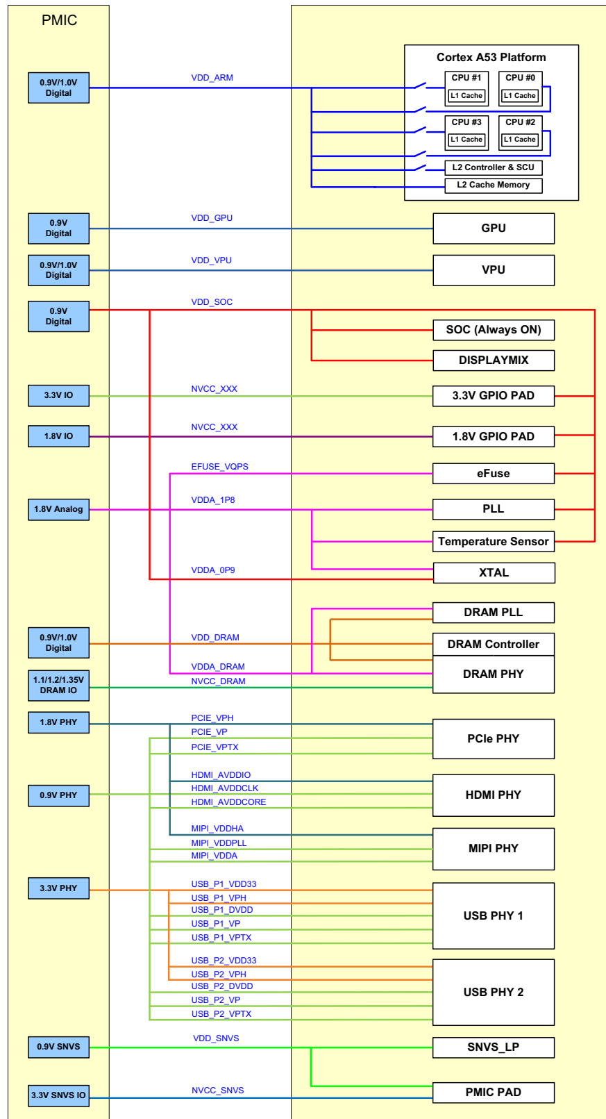
Figure 3. Power architecture
