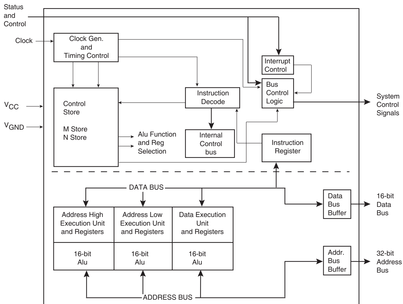
Figure 1-1. Block Diagram
