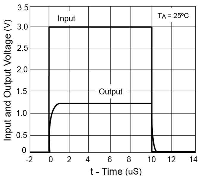
Figure 17: Pulse Response
