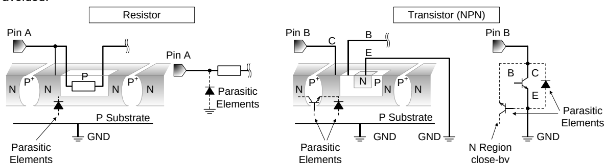
Figure 36. Example of IC Structure
