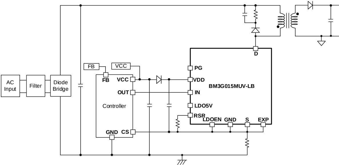
Figure 6. Flyback Converter Application Example
