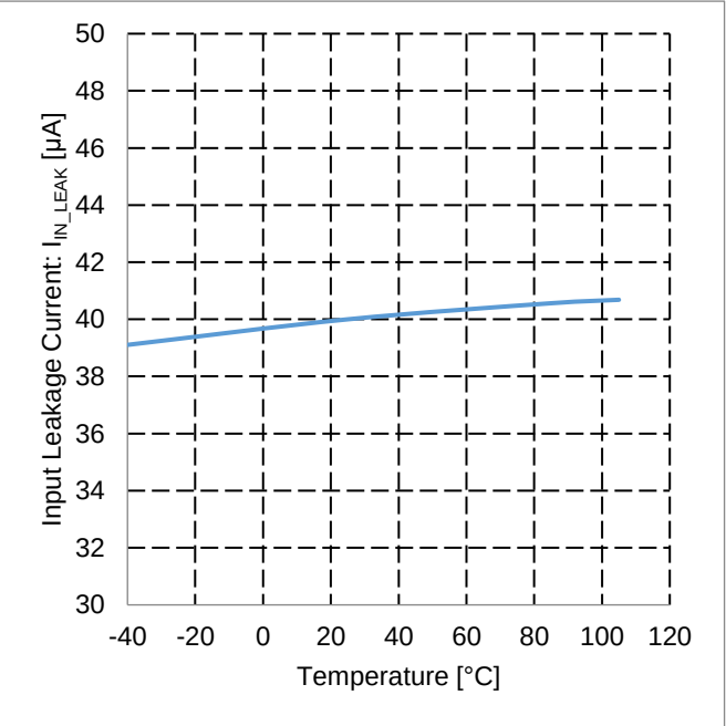
Figure 27. Input Leakage Current vs Temperature
