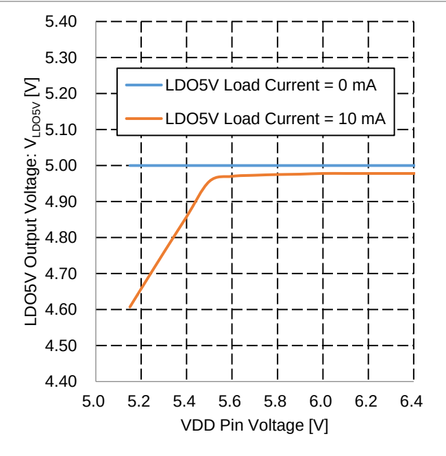
Figure 22. LDO5V Output Voltage vs VDD Pin Voltage
