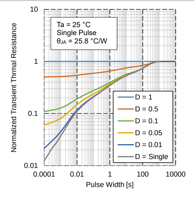
Figure 34. Normalized Transient Thermal Resistance vs Pulse Width
