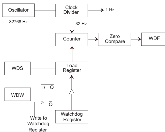
Figure 6. Watchdog Timer Block Diagram
