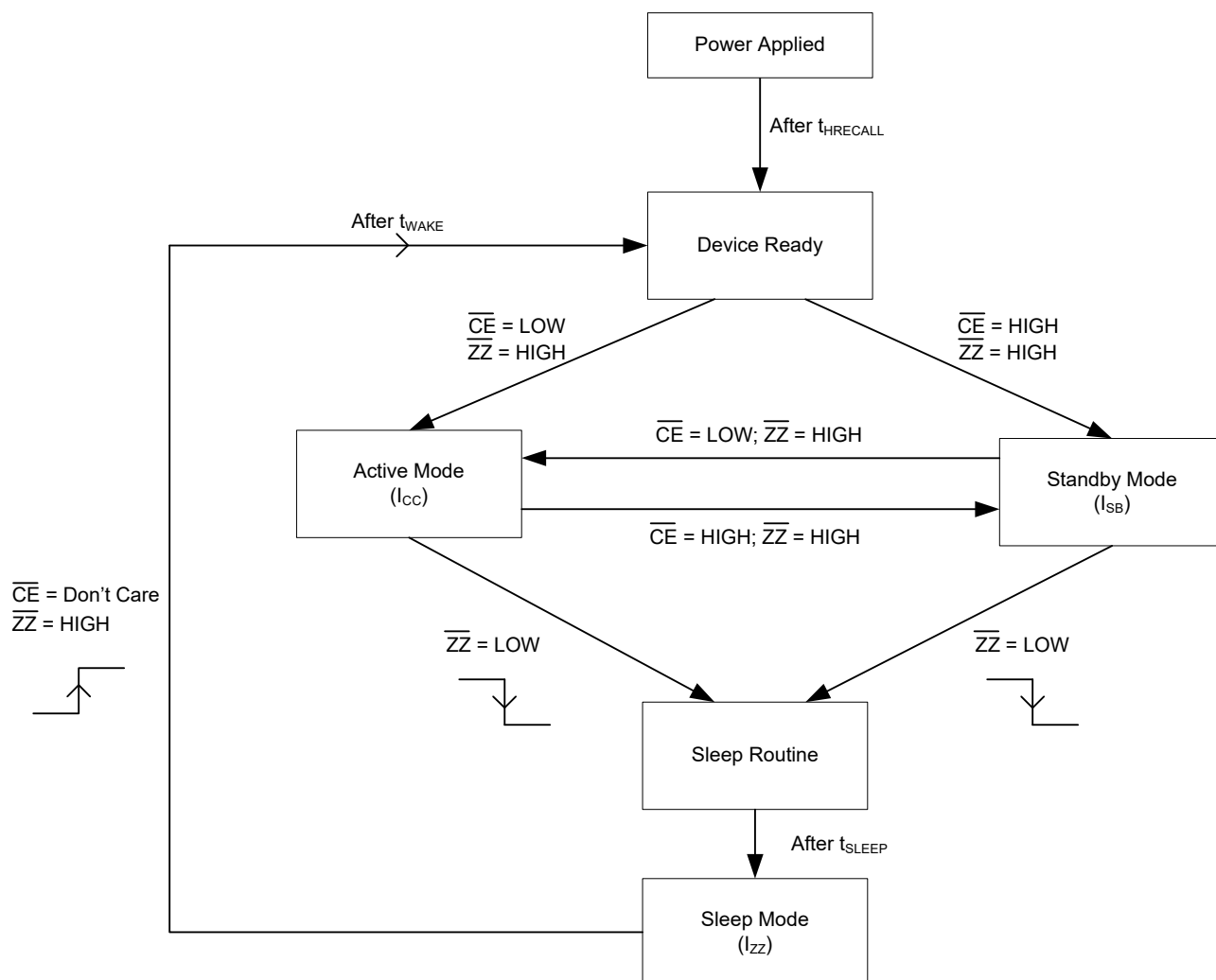
Figure 5. Sleep Mode ( \overline{ZZ} ) Flow Diagram
