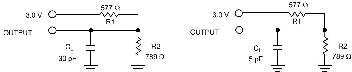
Figure 10. AC Test Loads and Waveforms
