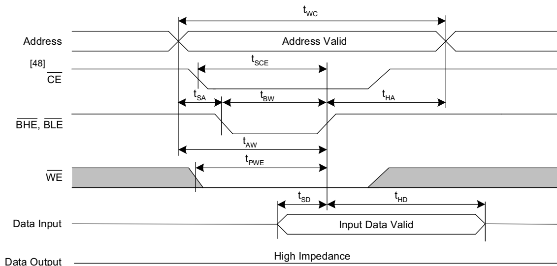
Figure 16. SRAM Write Cycle 3: \overline{\text{BHE}} , \overline{\text{BLE}} Controlled [44, 45, 46, 47, 49] (Not applicable for RTC register writes)
