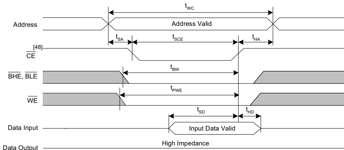
Figure 15. SRAM Write Cycle 2: \overline{\text{CE}} Controlled [44, 45, 46, 47]
