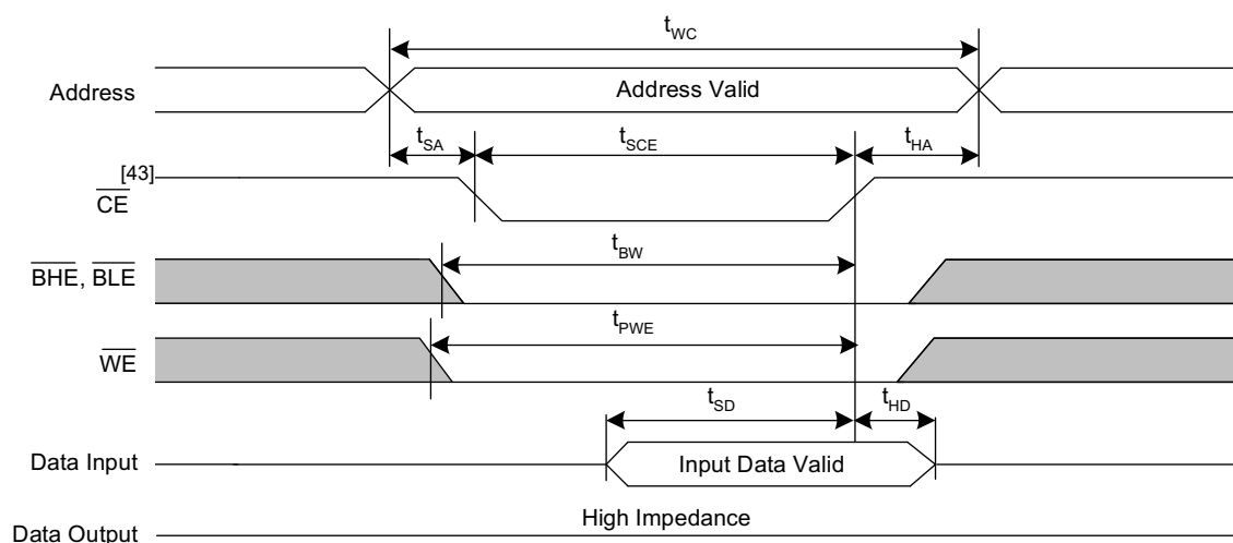
Figure 14. RAM Write Cycle 2: \overline{CE} Controlled [39, 40, 41, 42]
