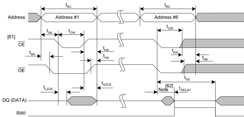
Figure 20. AutoStore Enable and Disable Cycle
