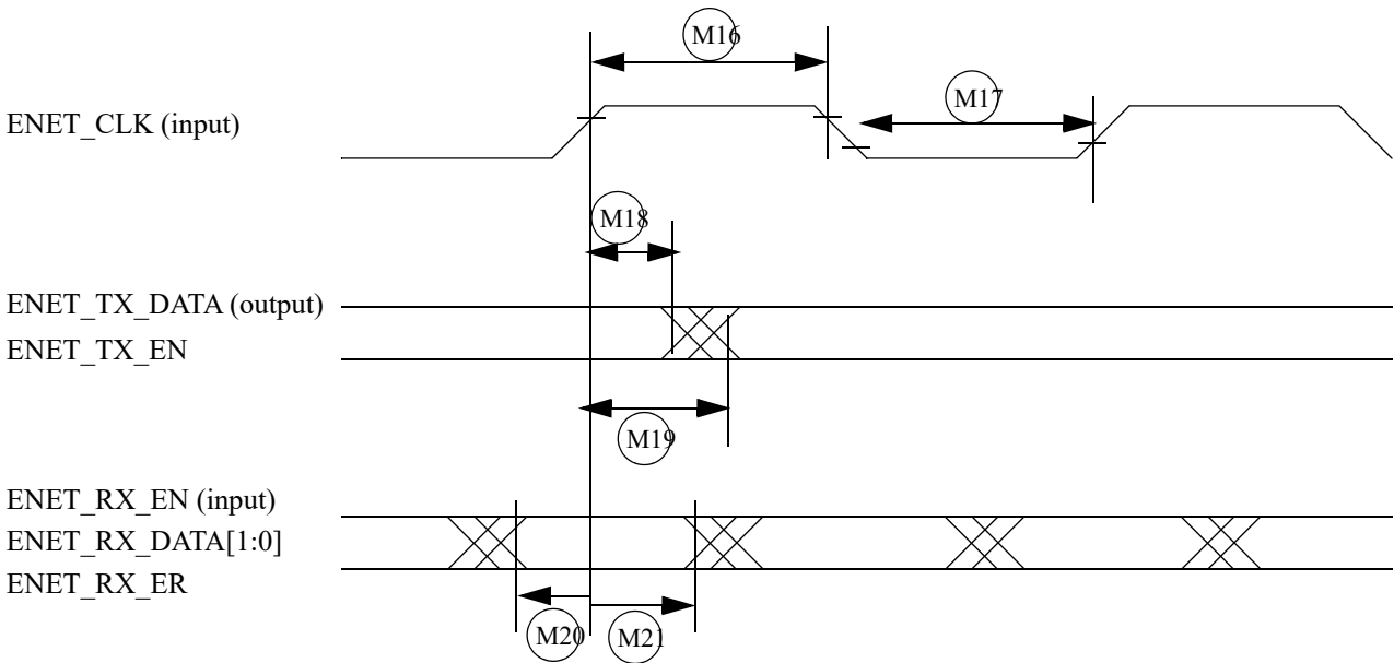
Figure 24. RMII mode signal timing diagram
