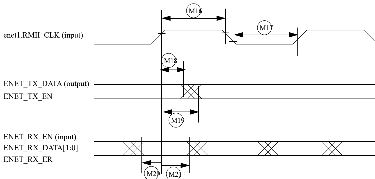
Figure 20. RGMII mode signal timing diagram
