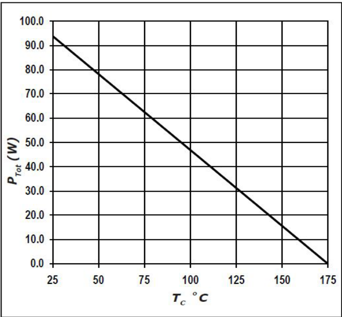
Figure 4 Power Derating
