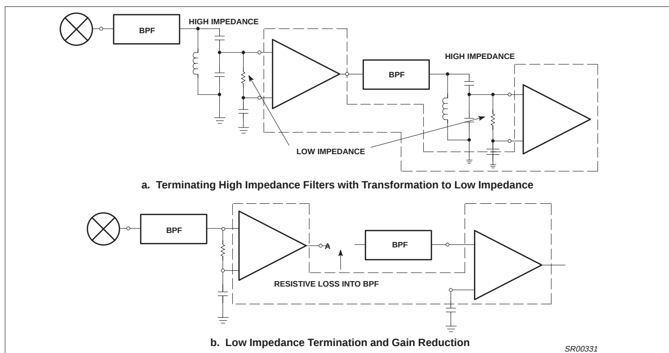
Figure 9. Practical Termination
