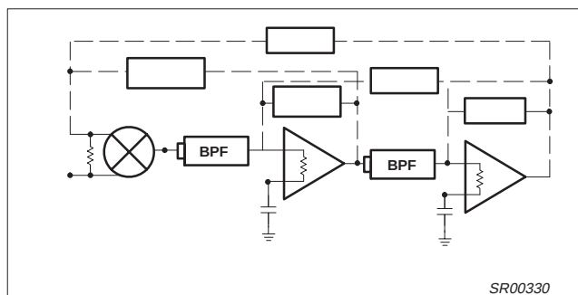
Figure 8. Feedback Paths
