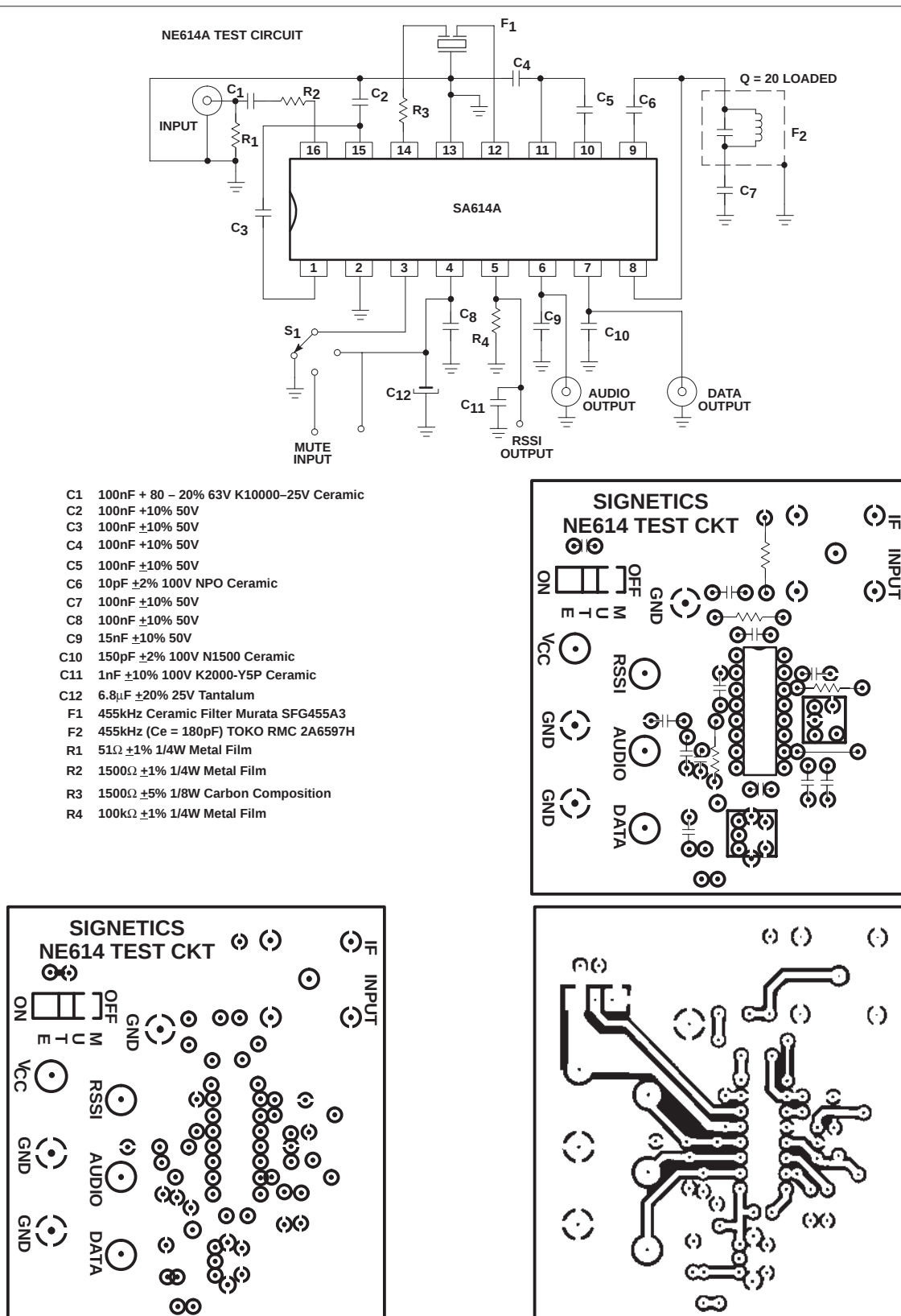
Figure 3. SA614A Test Circuit
