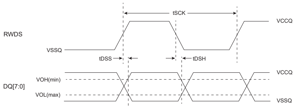
Figure 10.8 DDR output timing reference levels
