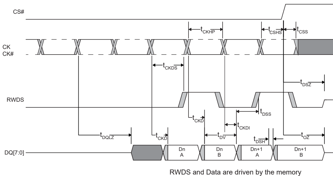
Figure 10.5 Read Timing Diagram - Data Valid Timing
