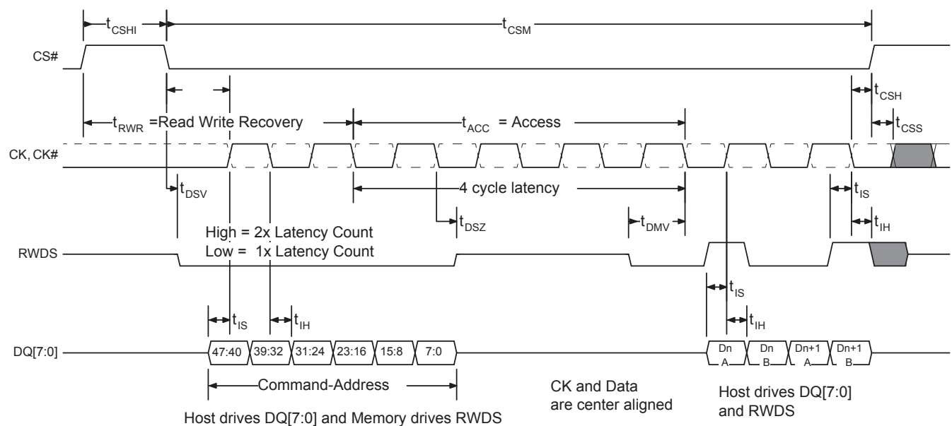
Figure 10.6 Write Timing Diagram — No Additional Latency
