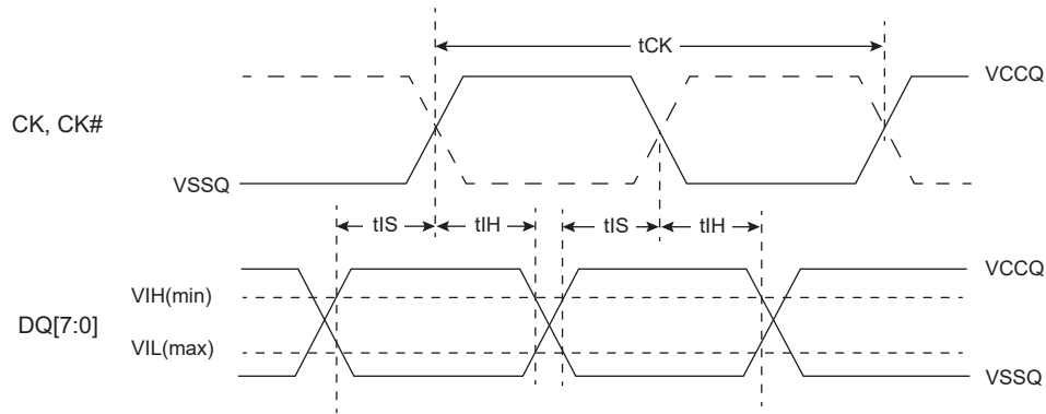
Figure 10.7 DDR input timing reference levels
