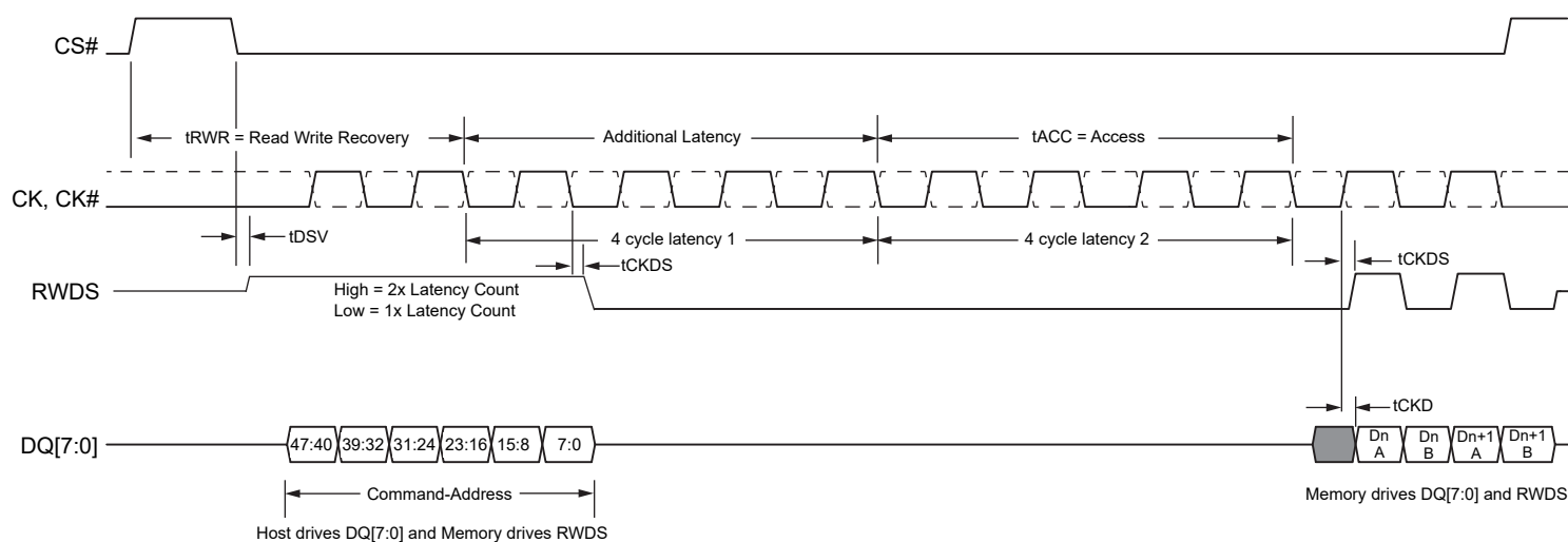
Figure 10.4 Read Timing Diagram - With Additional Latency Required
