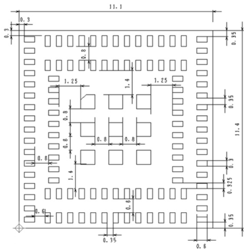
Figure 7.1 Recommended PCB Landing Pattern
