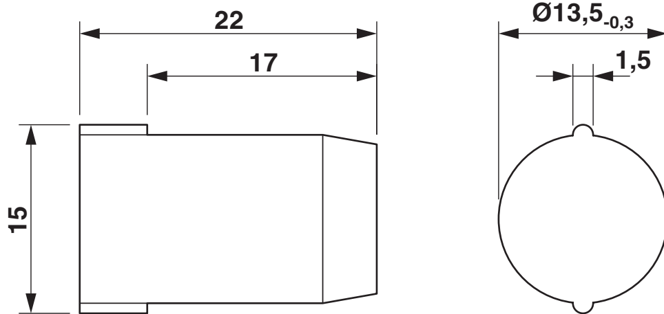
Dimensional drawing
