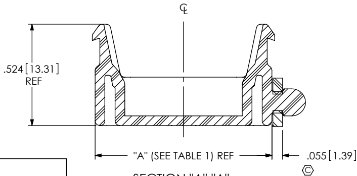
FIG. 1 DCA-RC5-10-01 SHOWN
