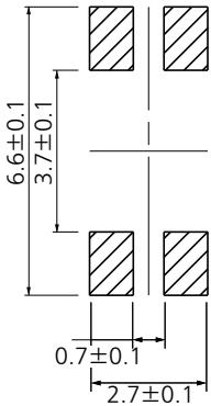
PWB land pattern for reference
