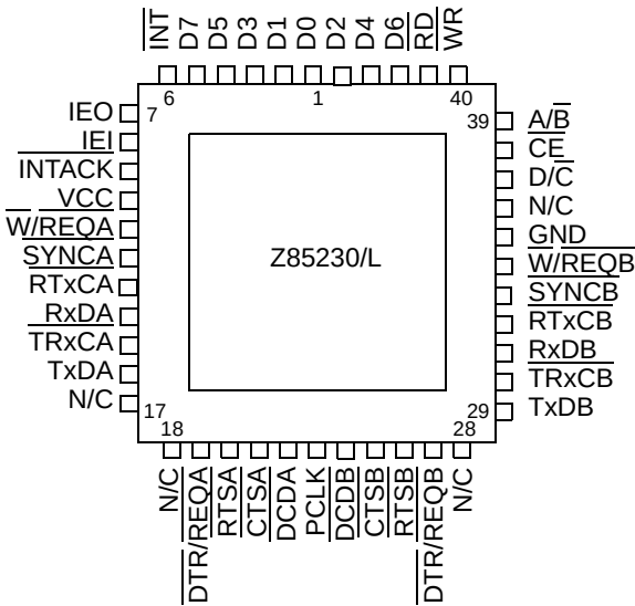
Z85230/L PLCC Pin Assignments
