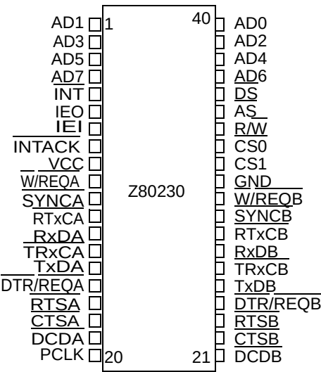
Z80230 DIP Pin Assignments
