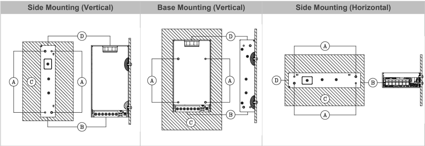
Fig. 2 Mounting Orientation
