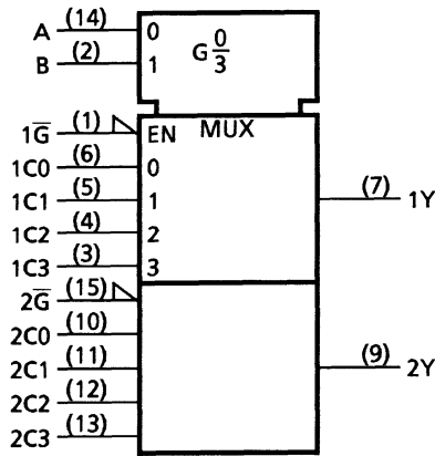
TC74HC153A
