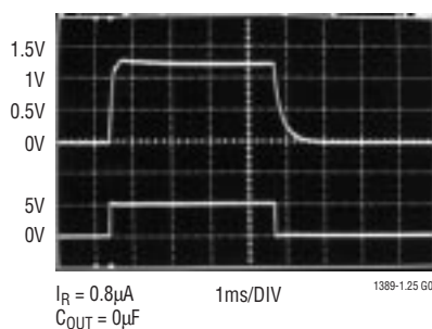
Response Time
