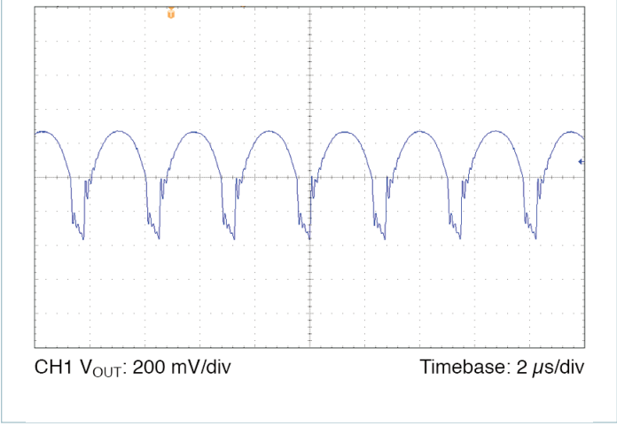
Figure 16 — Output voltage ripple, V_{IN} = 270\text{ V} , V_{OUT} = 5.0\text{ V} , C_{OUT\_EXT} = 1000\text{ }\mu\text{F} , R_{LOAD} = 0.100\text{ }\Omega
