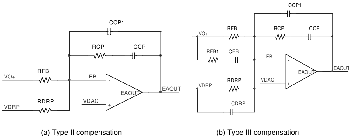
Figure 18. Voltage loop compensation network
