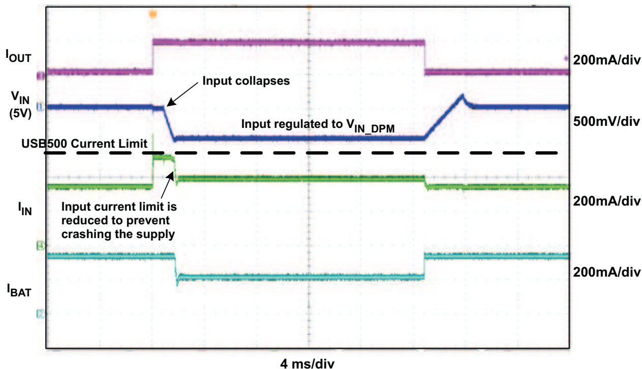
Figure 27. V_{IN\_DPM} Waveform
