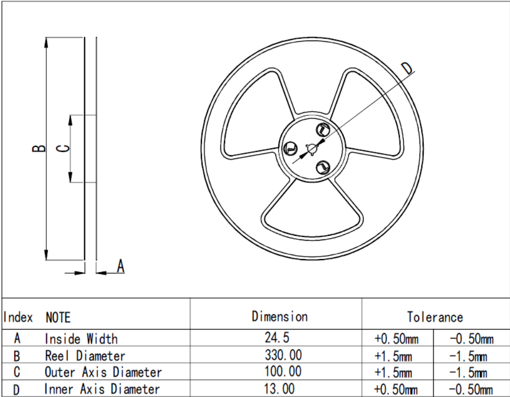
Figure 13. Reel Dimensions
