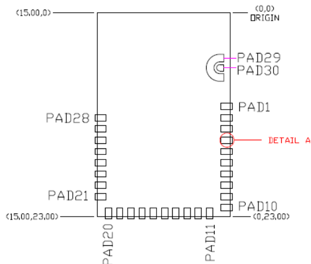
Top View (Seen on Host PCB)
